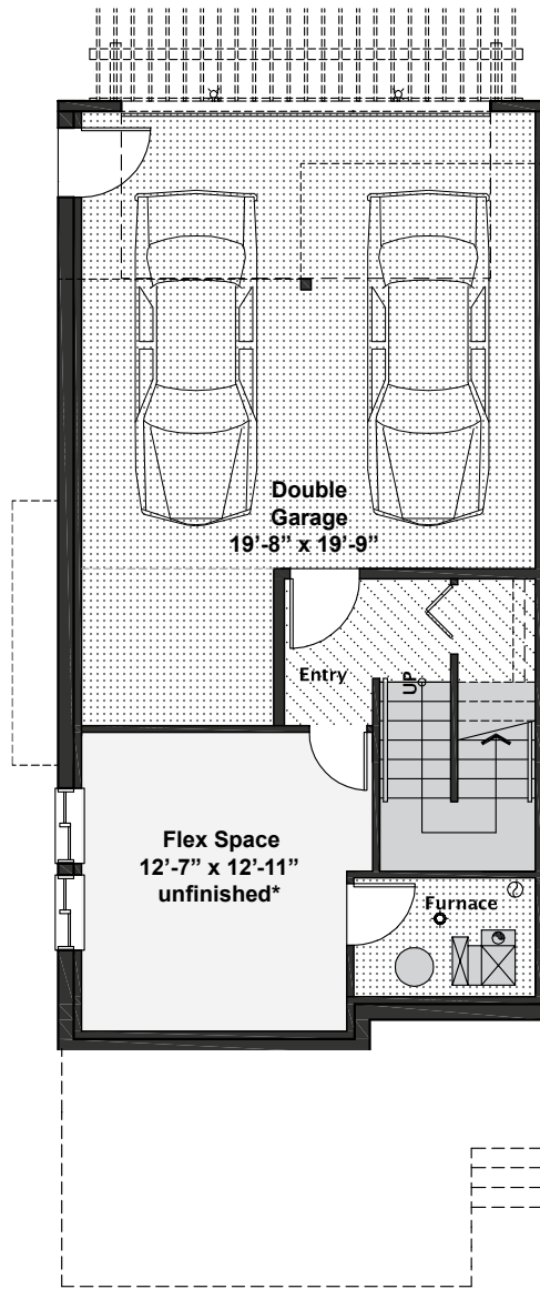
Ground Floor 206 sq.ft. *partially finished
