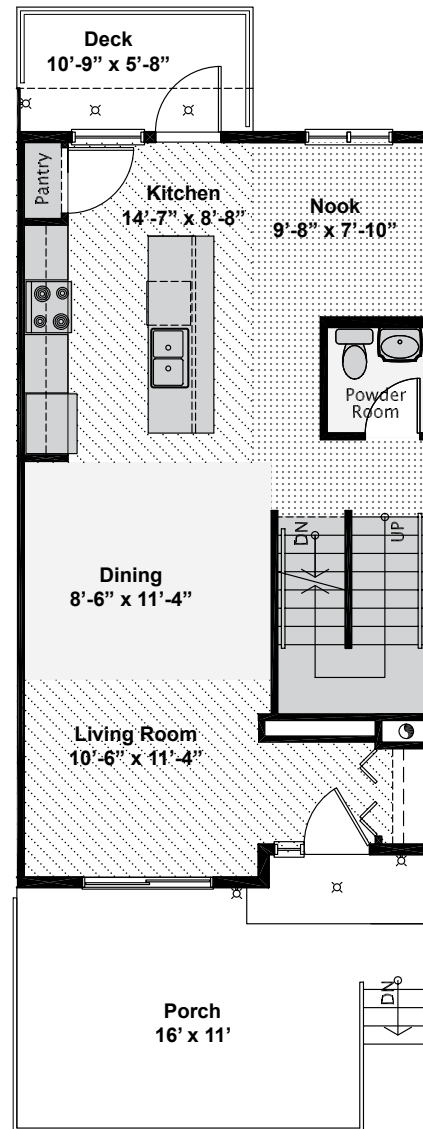
Main Floor Indoor Living 644 sq.ft. Outdoor Living 254 sq.ft.
