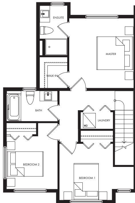
LEVEL 3
